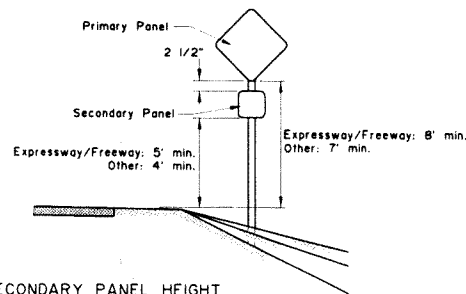
SECONDARY PANEL HEIGHT ALL TWO PANEL MOUNTING
