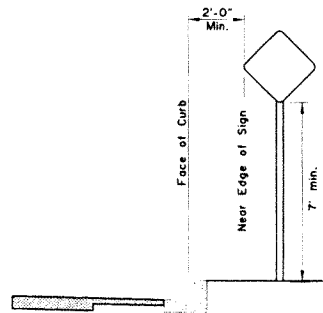
CURB WITHOUT SIDEWALK
