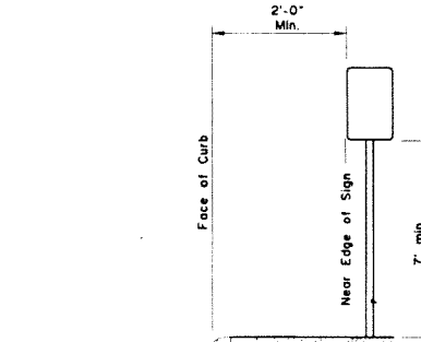
CURB WITH SIDEWALK WITHOUT PARKWAY
