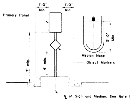
RAISED MEDIANS Minimum 4' Width for Signing
